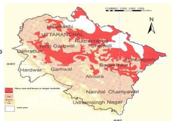
Chart-1.1.2 : Landslide hazard zonation of Uttarakhand
